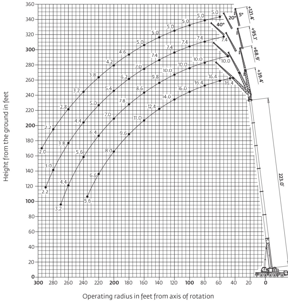
223 ft main boom with 39 ft and 69 ft swingaway
