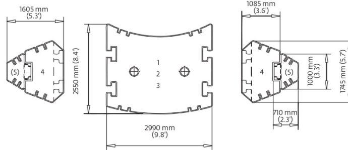
Counterweight Configuration kg (lb)
